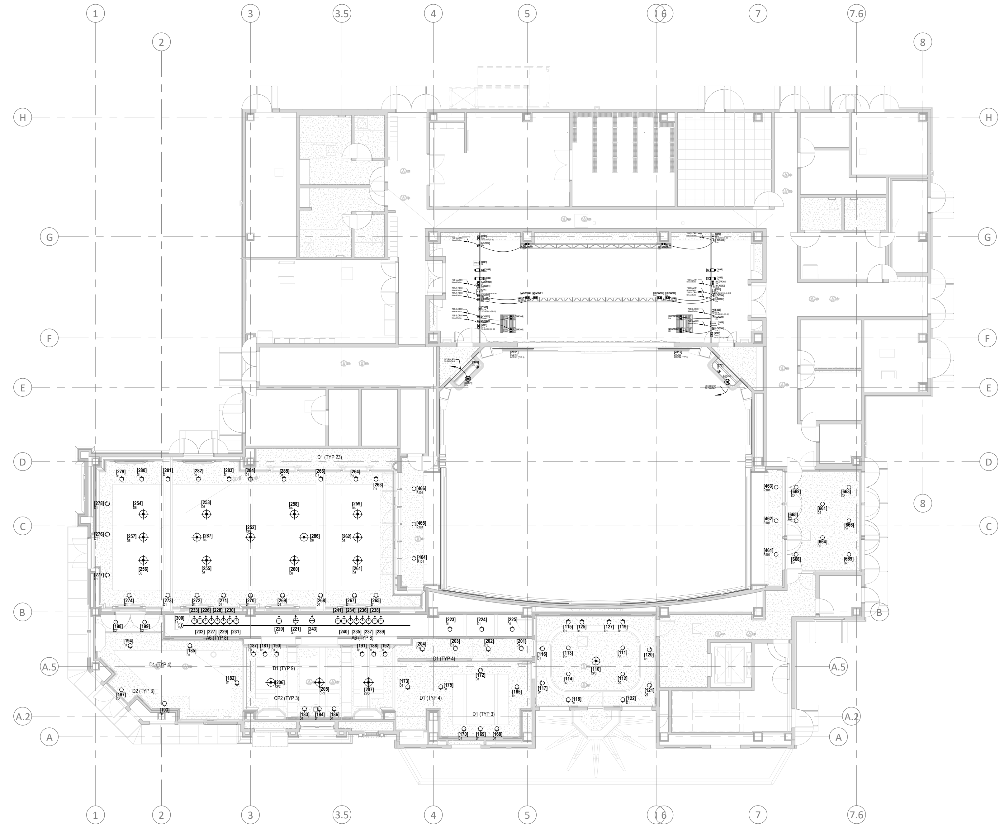
天花平面图-主题灯光 2 CEILING PLAN - THEMED LIGHTING TL131b
